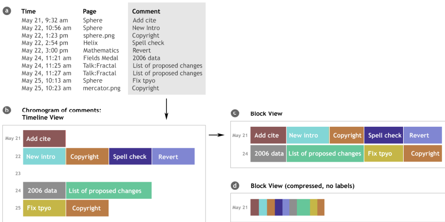
Fig. 2. Creating a Chromogram
