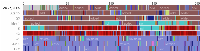
Fig. 15. Comment chromogram with about 2,000 edits between February and July 2005. Long-term task focus switches are evident. Brown: categorization; blue: reverts.
