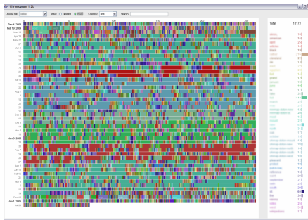
Fig. 3. The Chromogram Application: Block View
